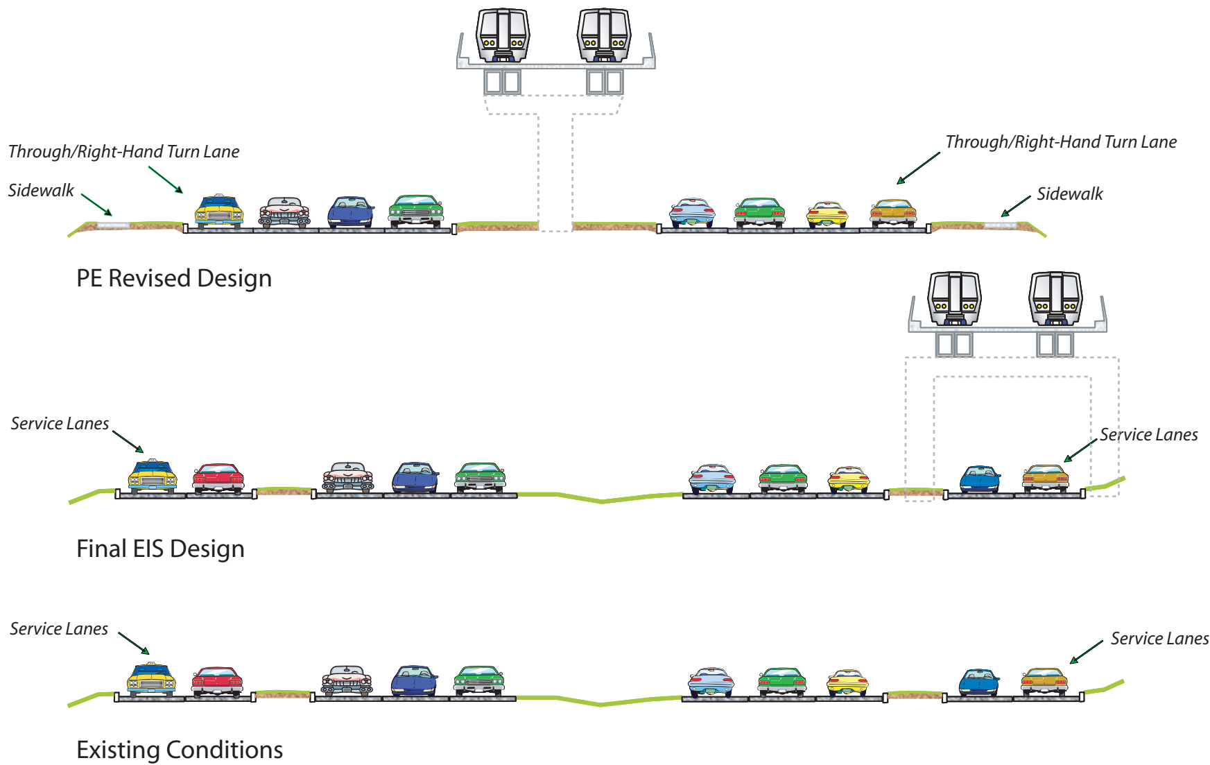
Figure 2-5 Proposed Cross-Section Changes along Route 7
