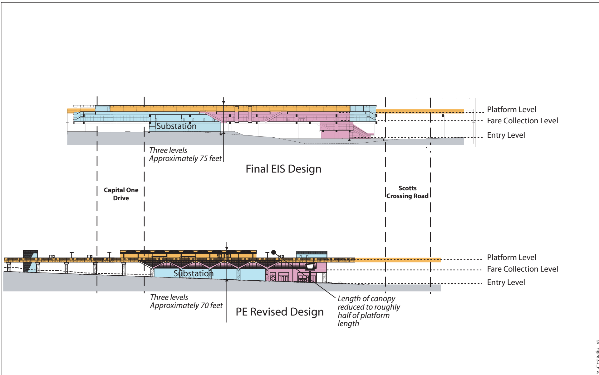
Figure 2-7 Tysons East Station Longitudinal Section
