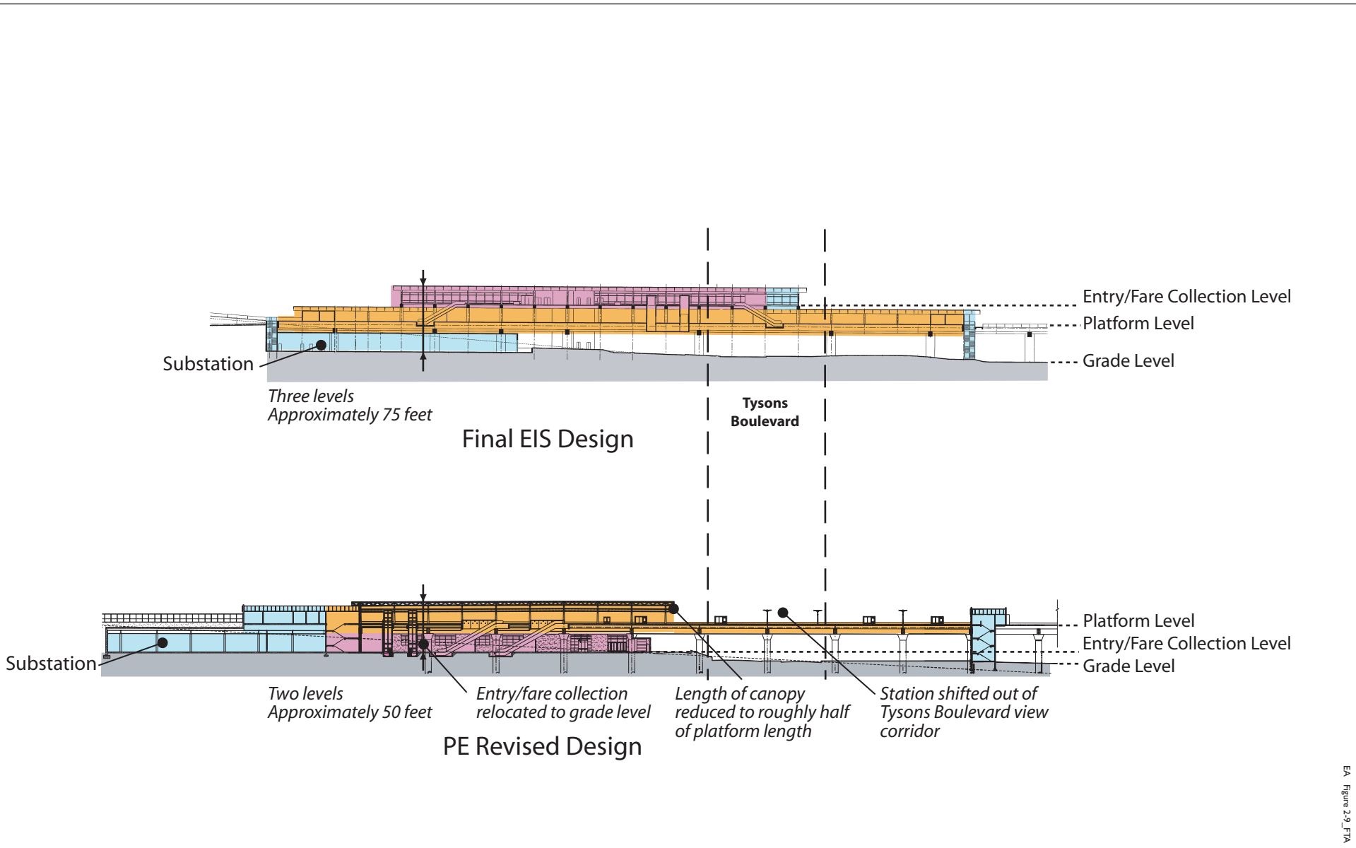
Figure 2-9 Tysons Central 123 Station Longitudinal Section
